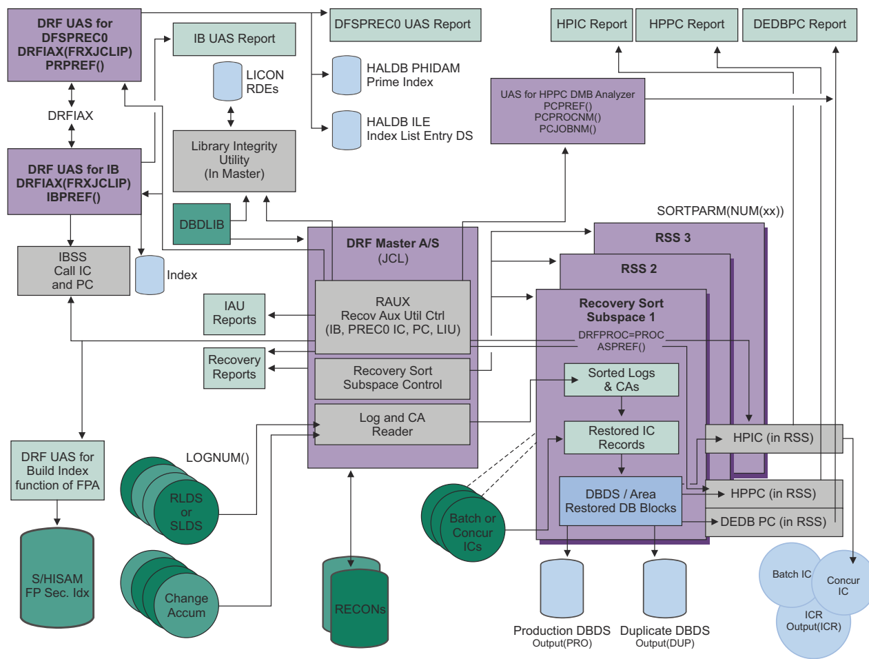
Figure 2. Integrated auxiliary utility processing with address spaces shown
